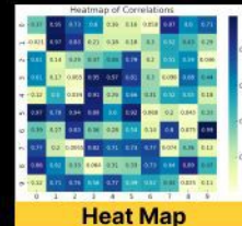
Heat Map
