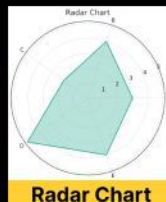
Radar Chart
