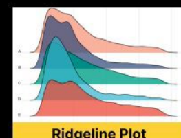
Ridgeline Plot
