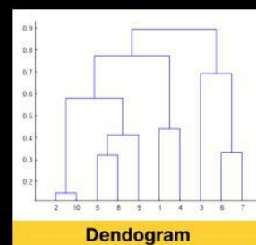
Dendrogram
