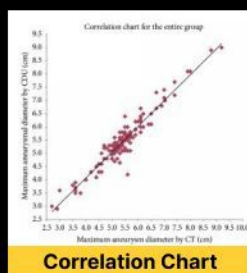
Correlation Chart
